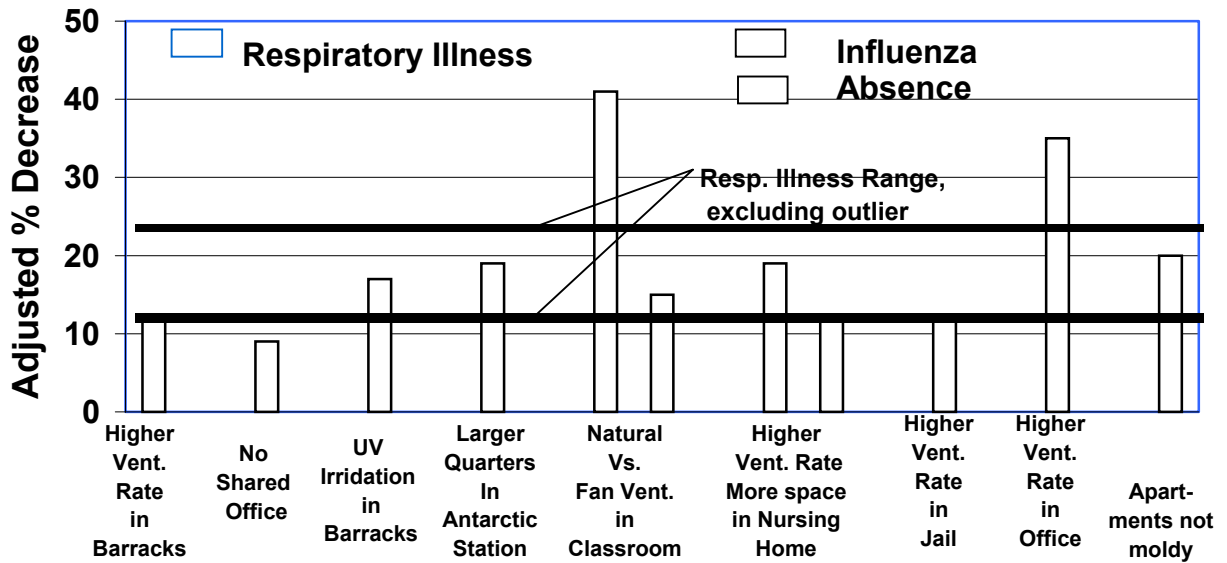
Figure 2. Estimated decreases in respiratory illness from changes in building characteristics.
